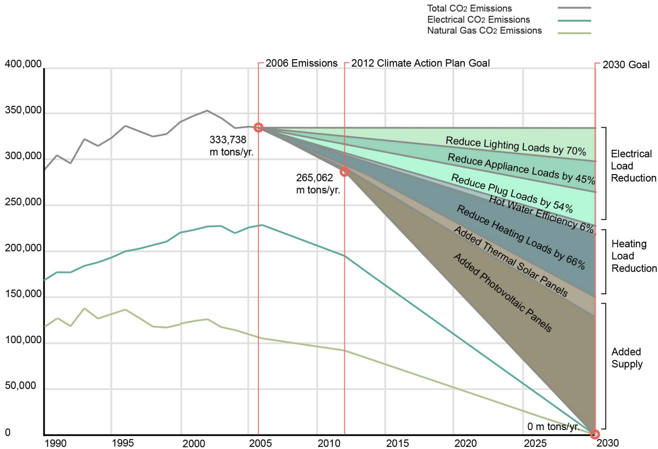
Total Boulder Residential CO 2 Emissions per Year Emissions Reduction Strategy
